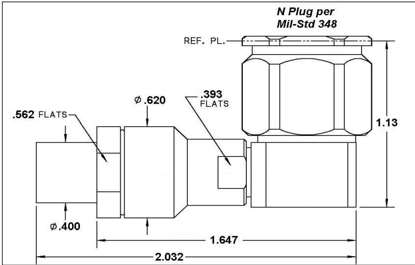
Features Not Shown : Safety Wire Holes, Gasket in Front
